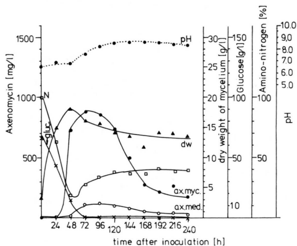
Fig. 13. Time course study of dry weight formation (dw), axenomyacin production in the medium (ax. med.) and mycelium (ax. myc.), amount of nitrogen (N) and glucose (gluc) in the medium and pH of the medium. The experiment was carried out with strain 3935-1-18-9 in medium 12.
